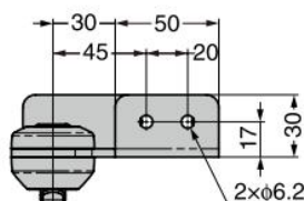
[HG-MA95A-L]
