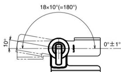
[HG-MA95A-L]
