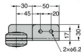
[HG-MA95AF-L]
